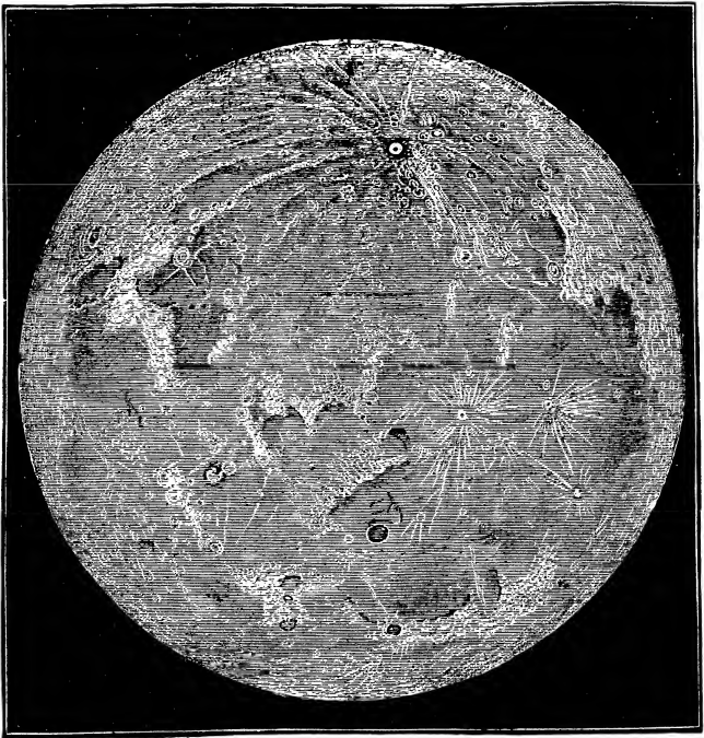
Fig. 38.—The Full Moon.
